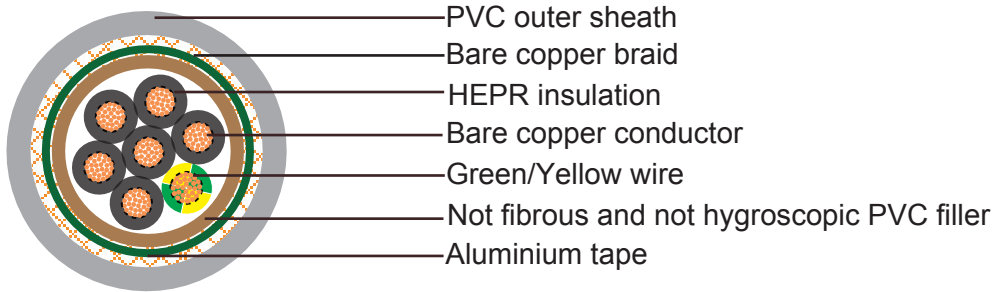
FG70HH2R
